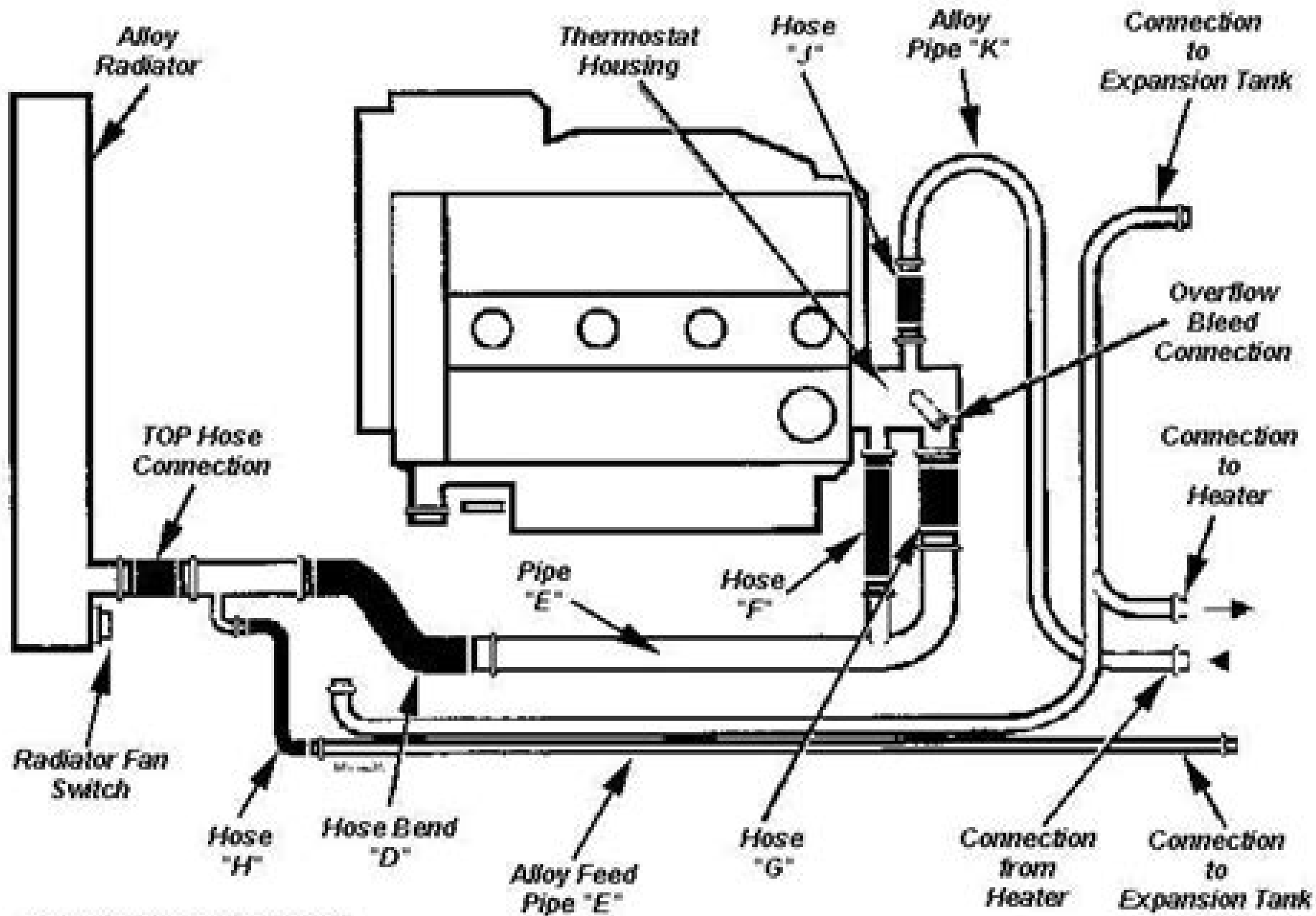
Diagram 52 (Ducted Nose)
