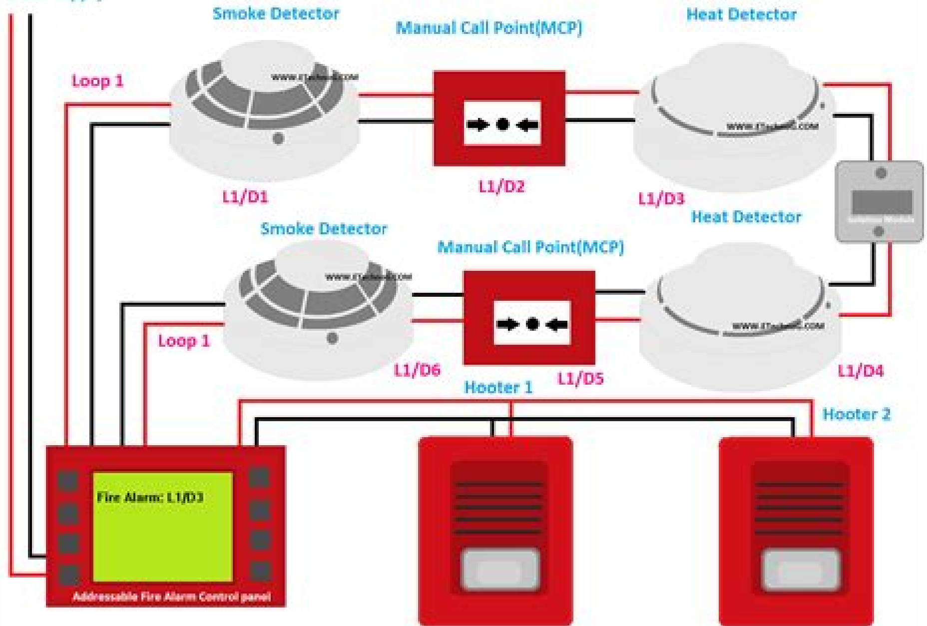
Addressable Fire Alarm System Wiring and Connection Diagram
