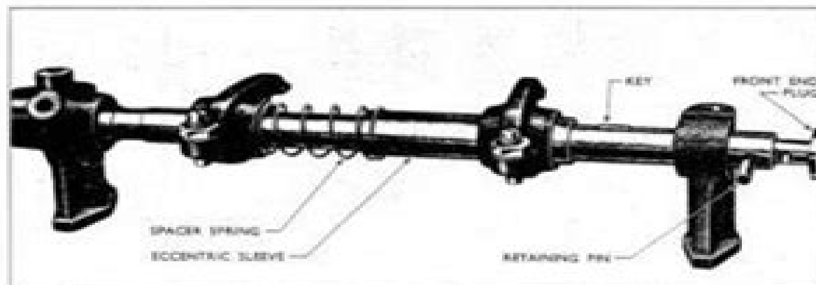
Fig. 2 Rocker Shaft and Supports
