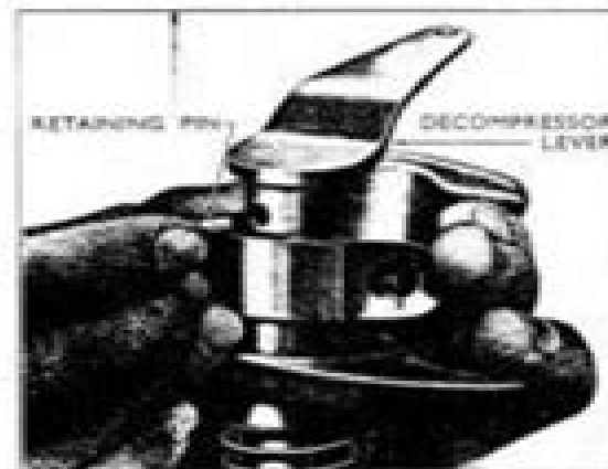
Fig. 3 Decompressor Lever
