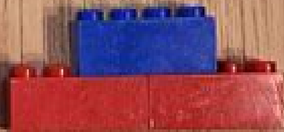
Nitrous oxide
