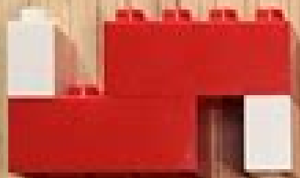
Hydrogen peroxide
