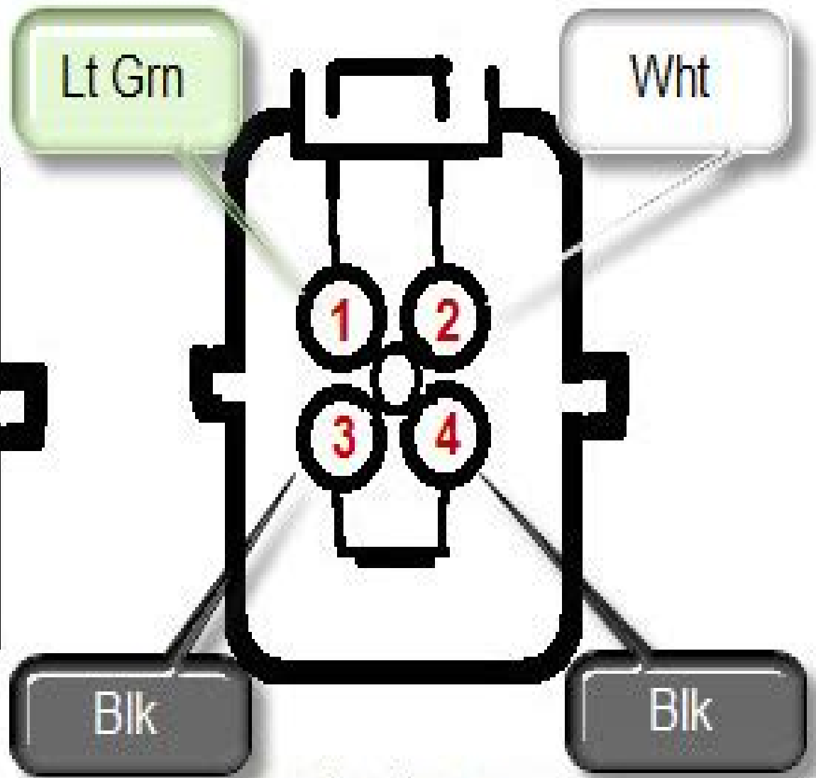
Back Side View
