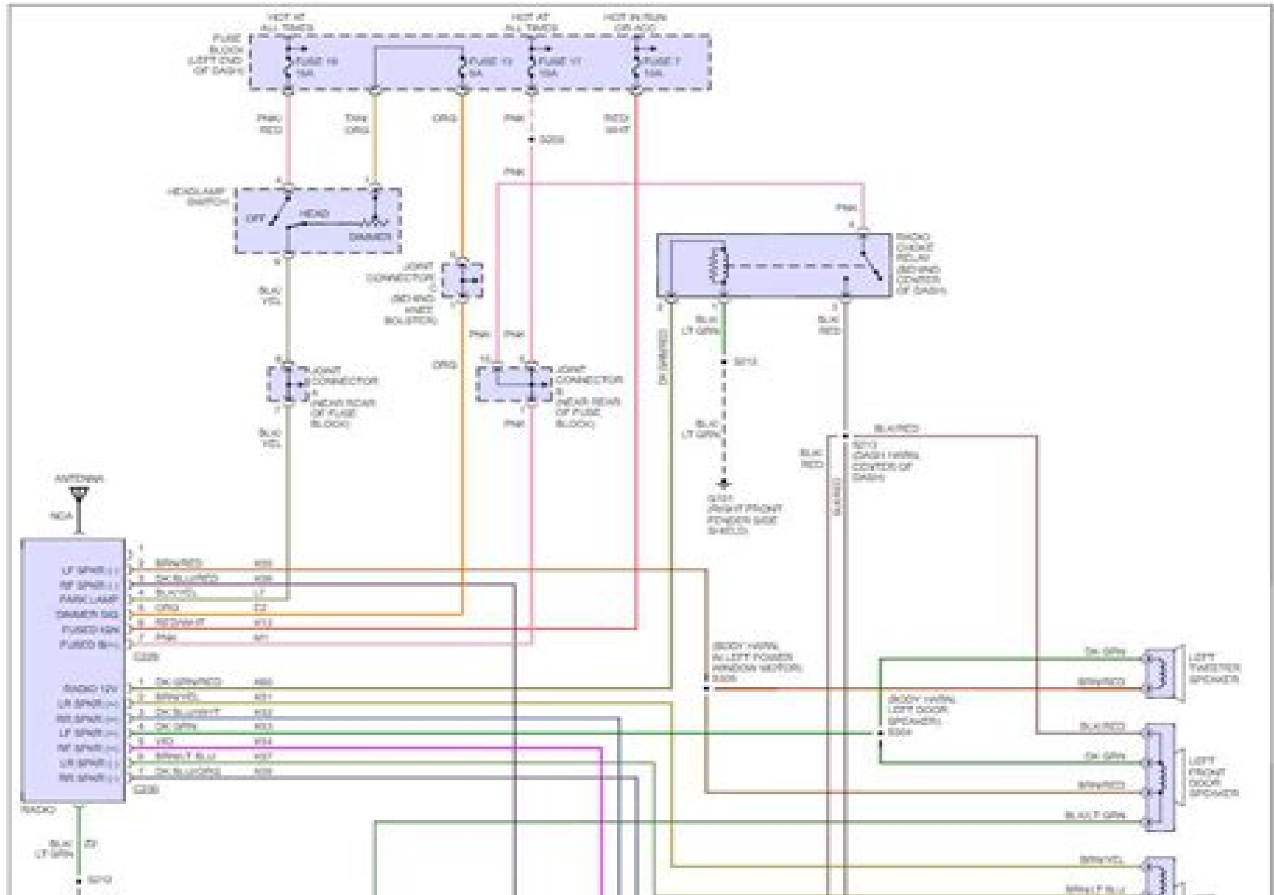
Fig 2: Radio Circuits, Premium Radio
