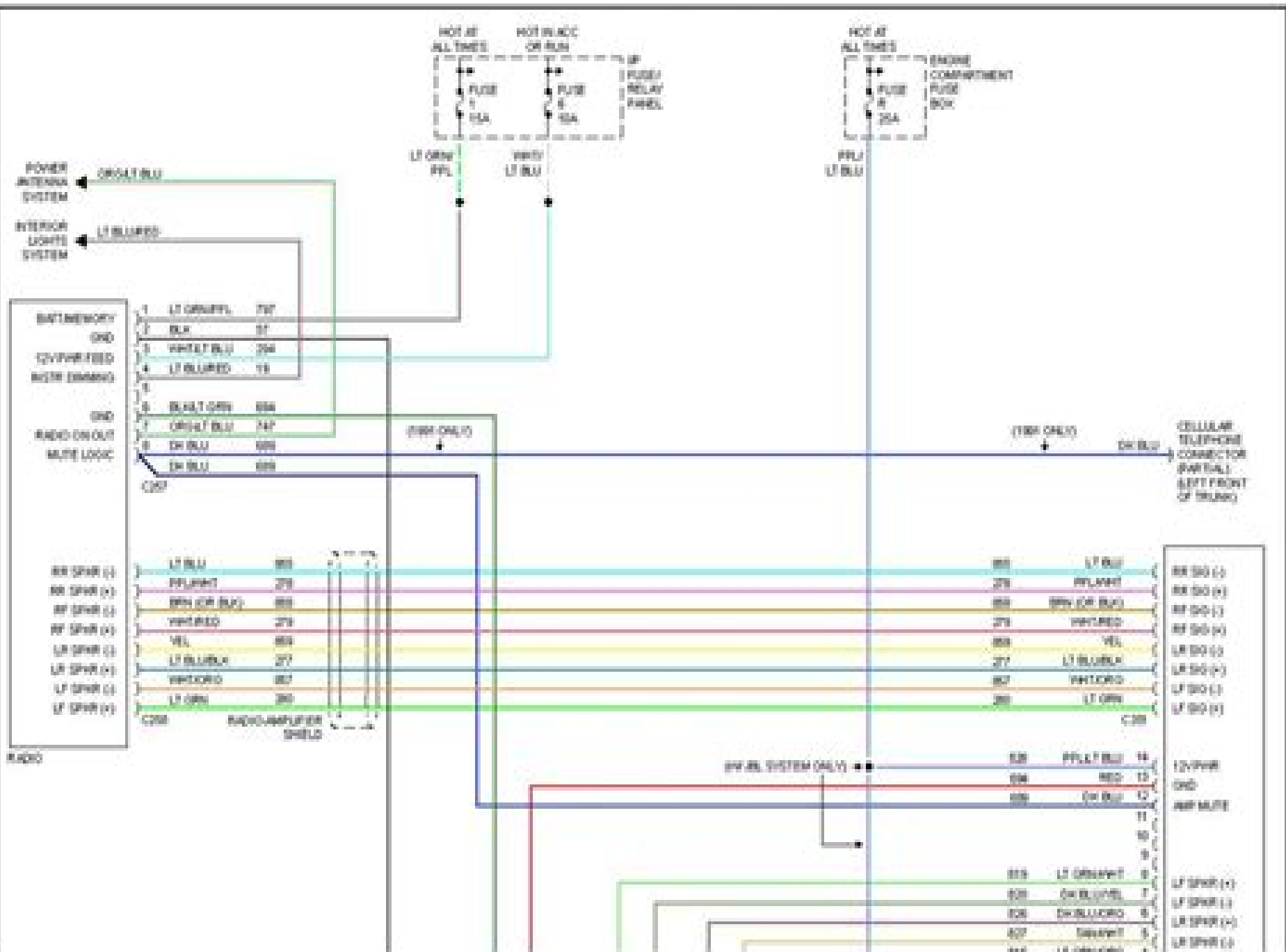
1990 Lincoln Town Car Fig. 1A Radio Circuits
