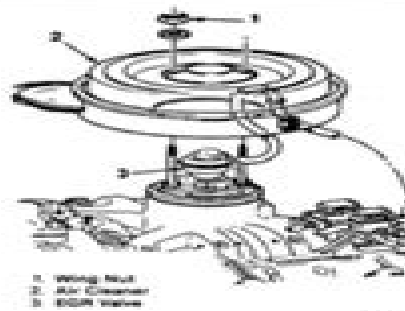
Fig. 30 Exploded view of the air cleaner housing—6.2L diesel engines
