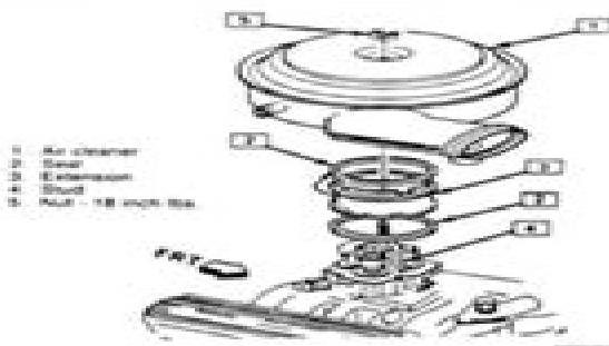
Fig. 28 Typical air cleaner housing assembly components—1985-92 gasoline engines
