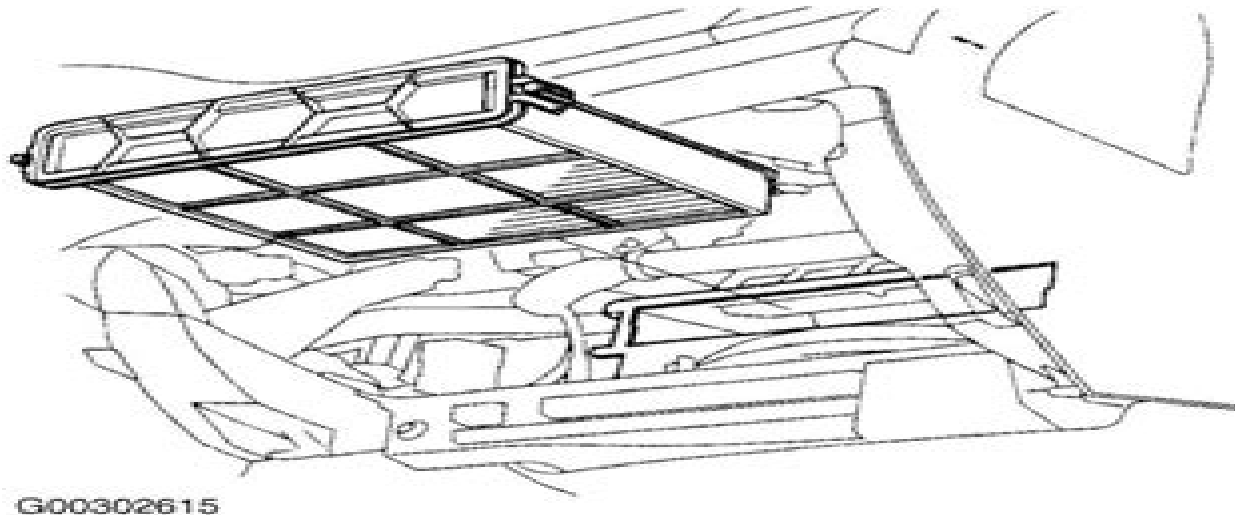
Fig. 1: Removing Dust & Pollen Filter From Evaporator Courtesy of AMERICAN HONDA MOTOR CO., INC.
