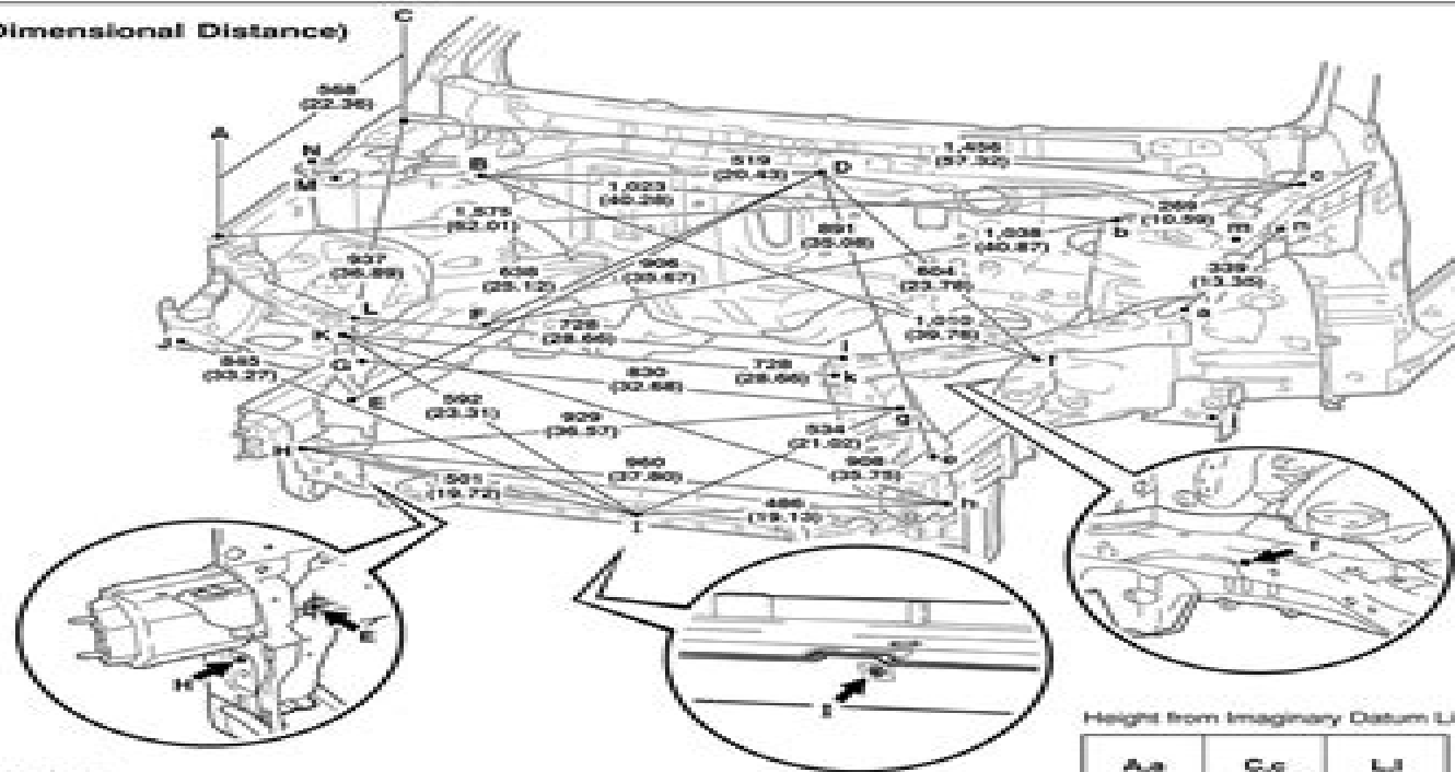
Vehicle Dimensions
