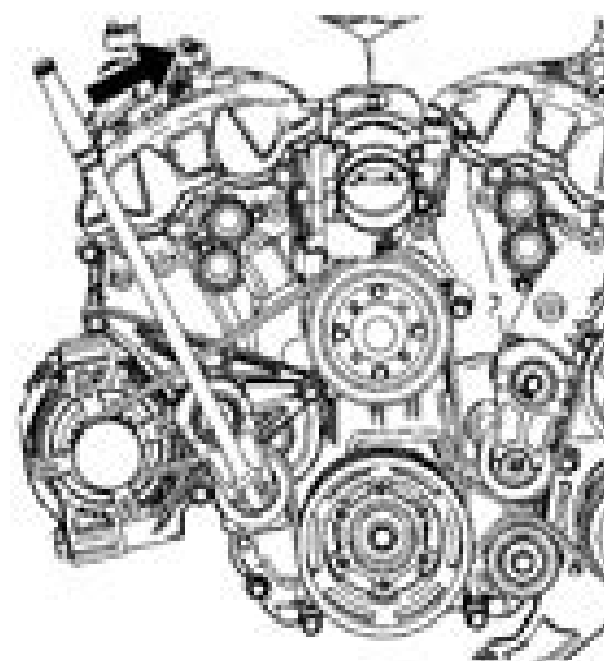
Fig. 1: Removing/Installing Generator & Water Pump Drive Belt Courtesy of GENERAL MOTORS CORP.
