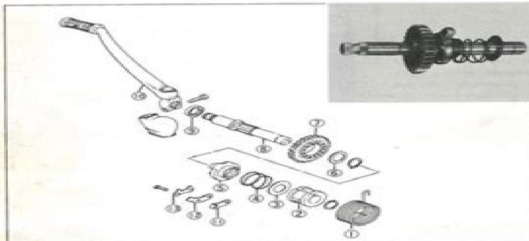
Fig. 82. Kick starter assembly (exploded)
