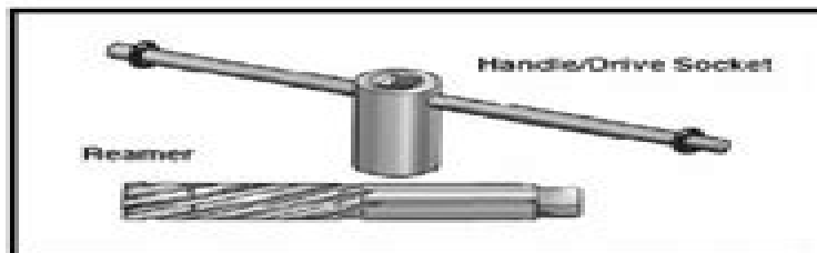
Figure 3-92. Connecting Rod Bushing Reamer (Part No. HD-423180) and Handle/Drive Socket (Part No. HD-436450)
