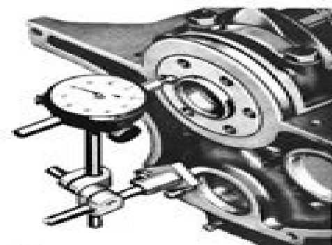
FIG. 5—Typical Crankshaft End Play
