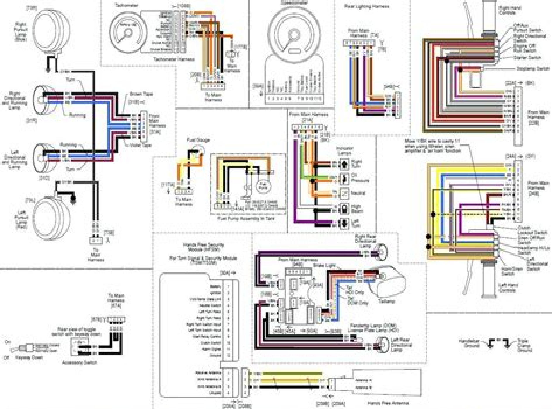
Figure A-15. Handfree Switches, Indicator Lamps, Tail Lamp, Power Lamps, Directional Lamps, Accessory/Reset Switch, Tachometer/Tachometer and IFM Antenna, 2008 FLTP and FLTPS, DOMESTIC and INTERNATIONAL Models
