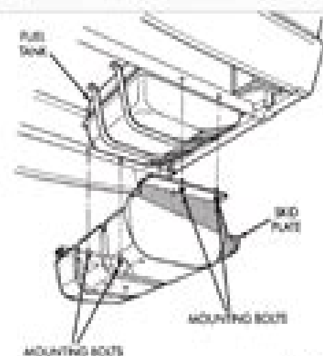
Fig. 2 Skid Plate—KJ Models
