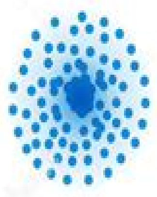
Quantum model
