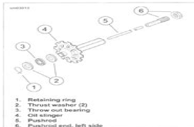
Figure 6-36. Pushrod Assembly: Cable Clutch
