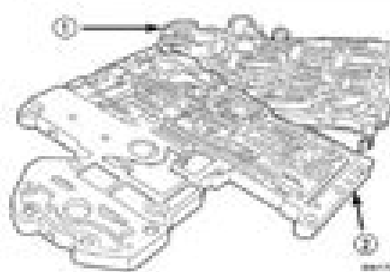
Fig. 305 Transfer Plate
