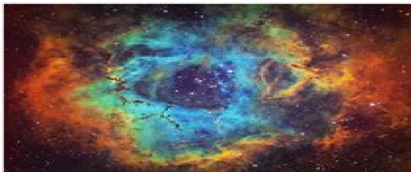
The Rosette Nebula
