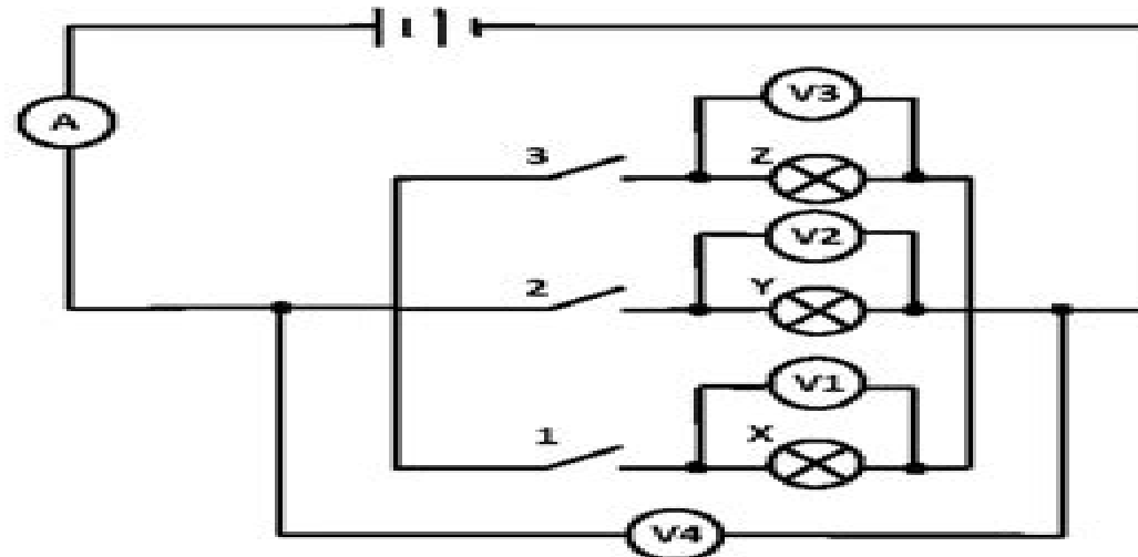
Circuit diagram 1
