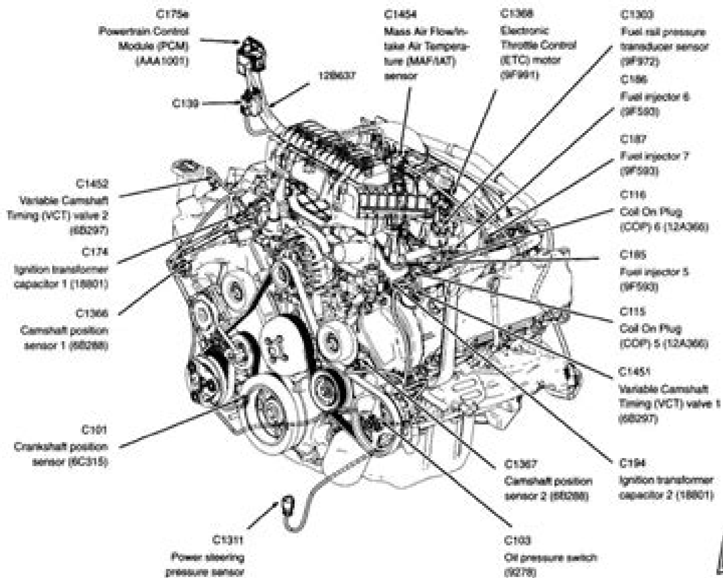
5.4L engine, front
