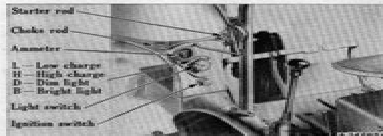
Illustr. 63—Light Switch, Ammeter, etc.
