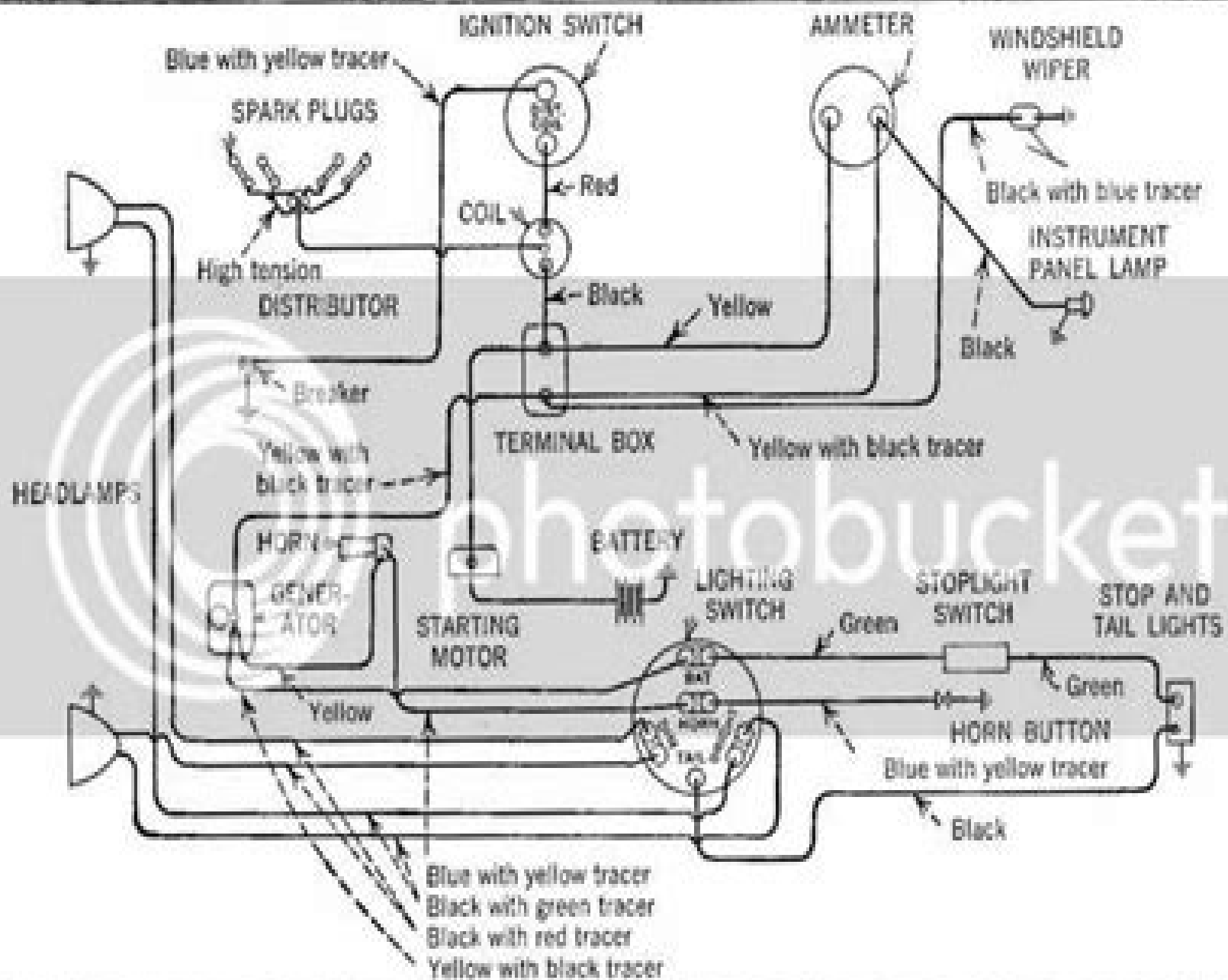
Fig. 28.—Wiring Diagram of the Ford Model A Showing All Units and Connections.
