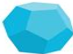
DODECAHEDRON
