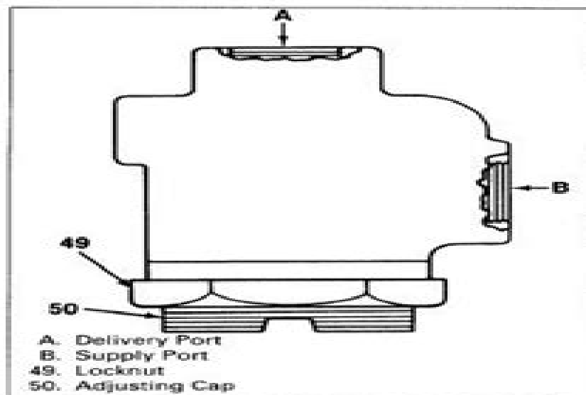
Figure 4 - Pressure Protection Valve
