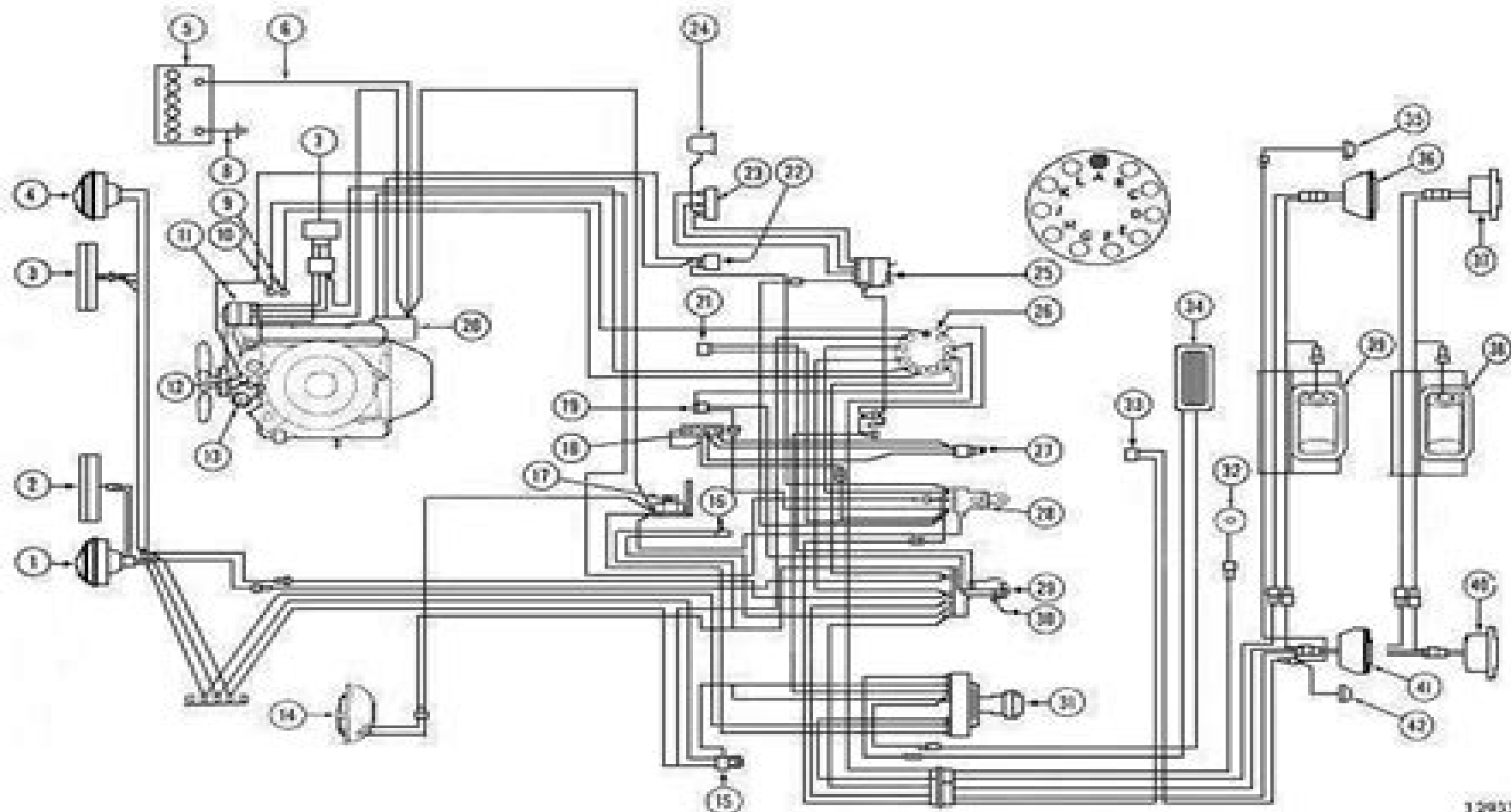
FIG. H-71—WIRING DIAGRAM, GLADIATOR TRUCK WITH V8-350 ENGINE
