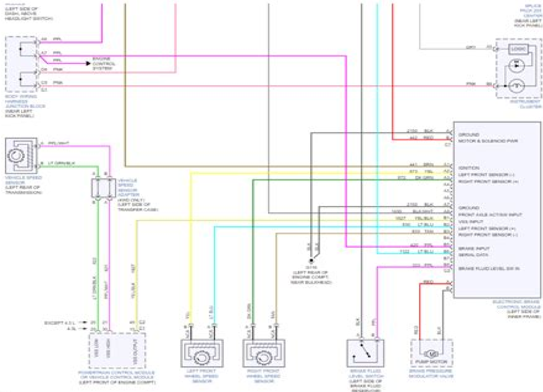
Fig 1: Anti-lock Brakes Circuit
