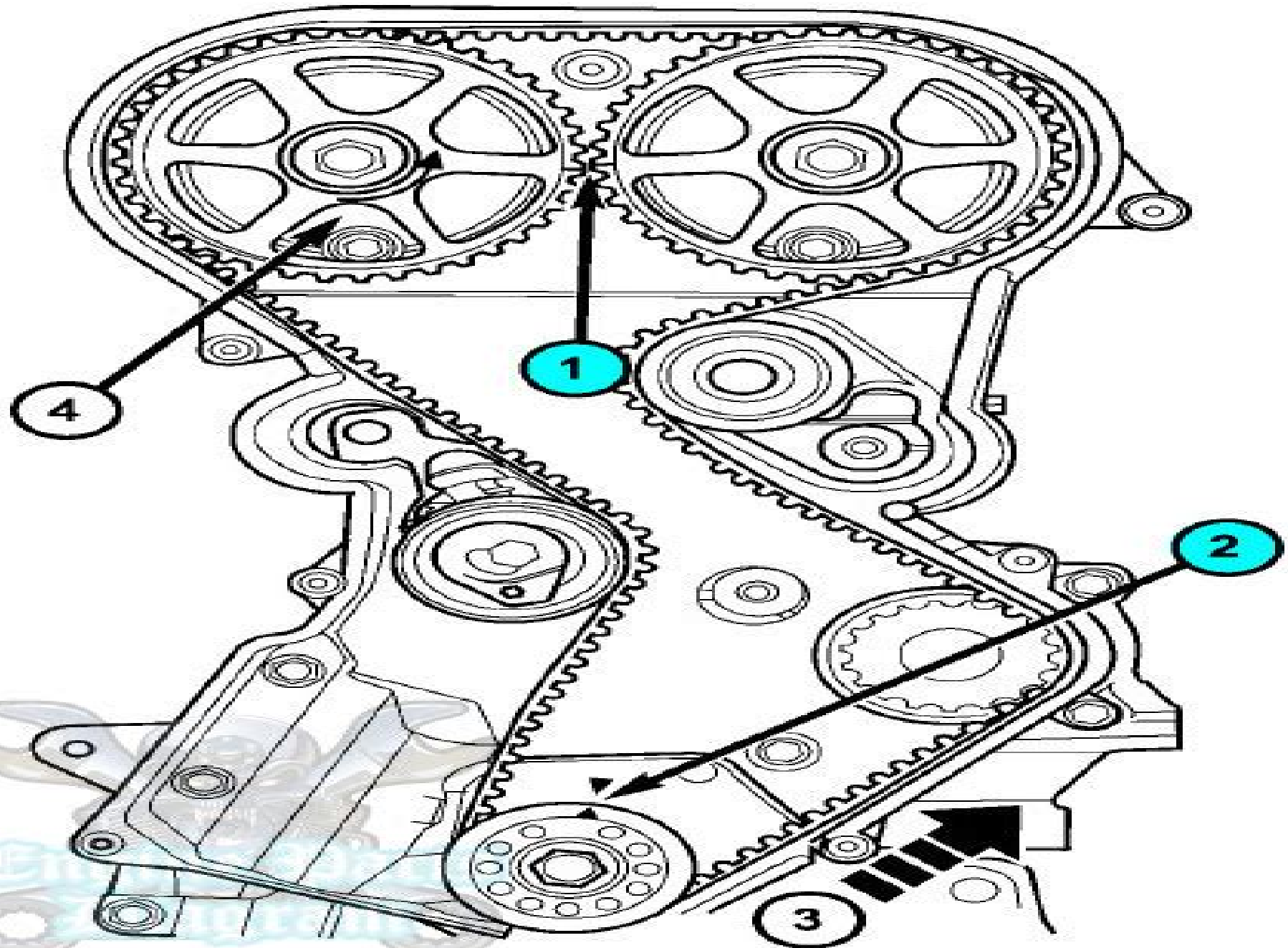
Chrysler 2.4L Engine Timing Marks
