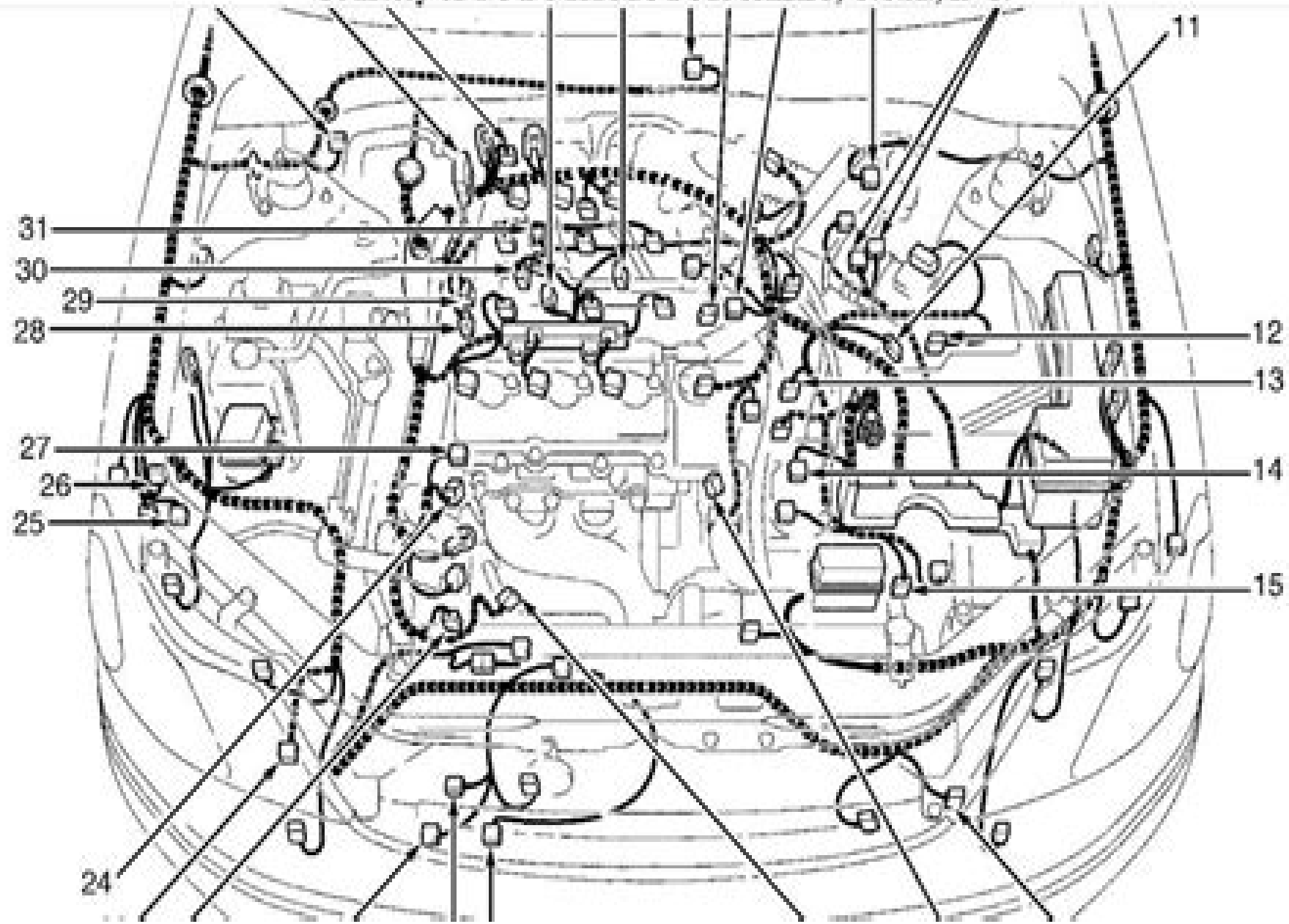
Fig. 1: Engine Compartment
