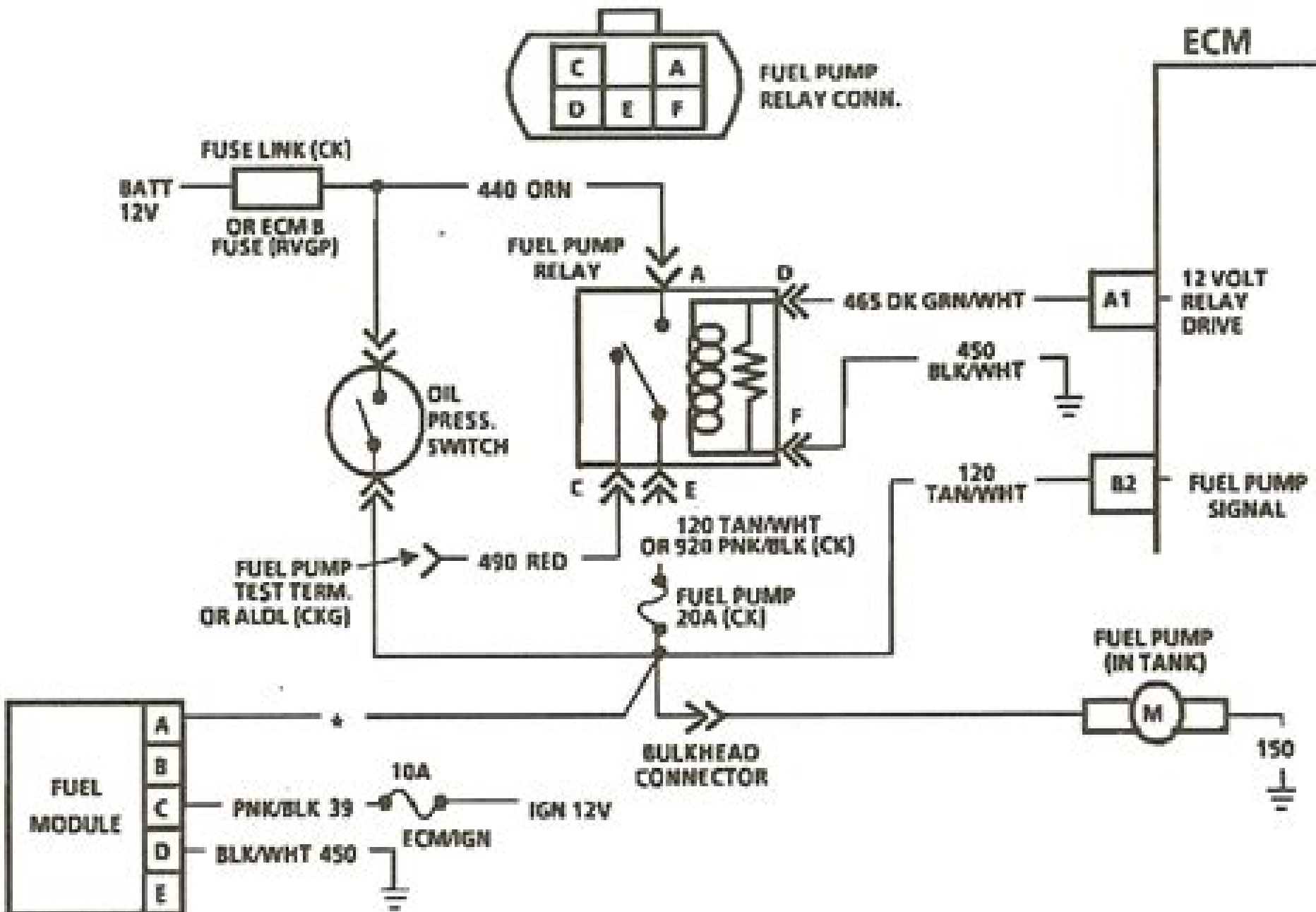
Wiring Diagram For Chart A-5 - Fuel Pump Relay Circuit Diagnosis (One Fuel Tank)
