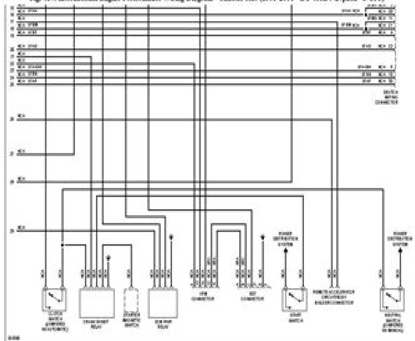
Fig. 417: International Engine Performance Wiring Diagram - Chassis Side (1995-2000) - DT 466E Navpack - 3 OF 3
