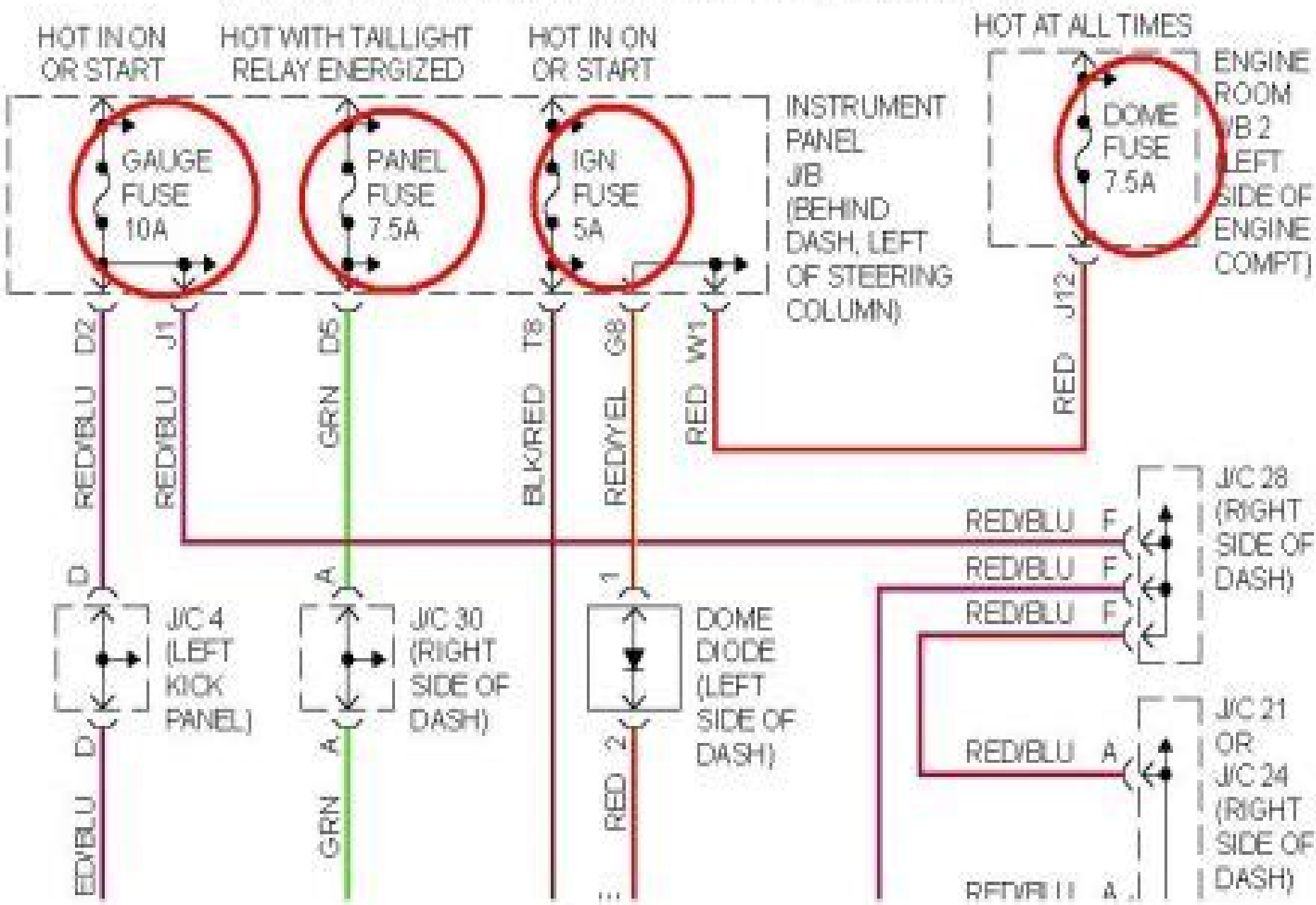
1998 Toyota Camry LE-Fig. 25: Instrument Panel Wiring Diagram (Camry - 1 Of 2)
