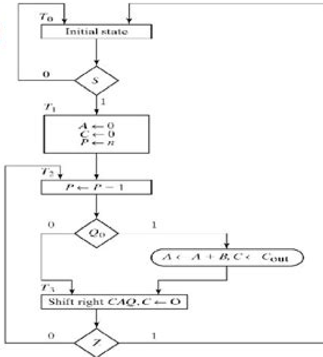
Fig. 8-14 ASM Chart for Binary Multiplier
