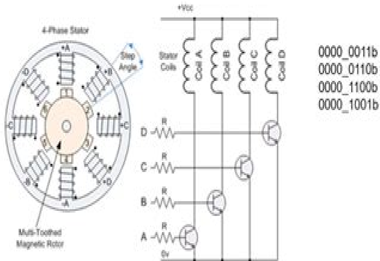
Figure 1: Variable Reluctance
