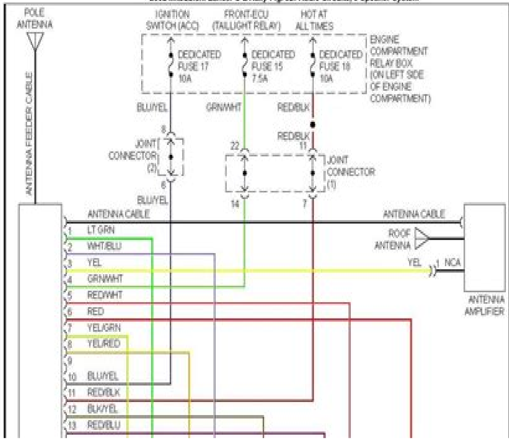
2002 Mitsubishi Lancer O-2 Rally-Fig. 32: Radio Circuits, 4-Speaker System
