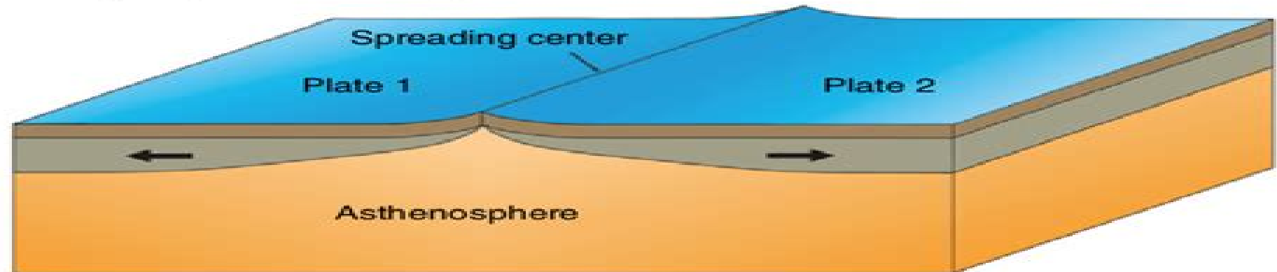
Divergent plate boundary
