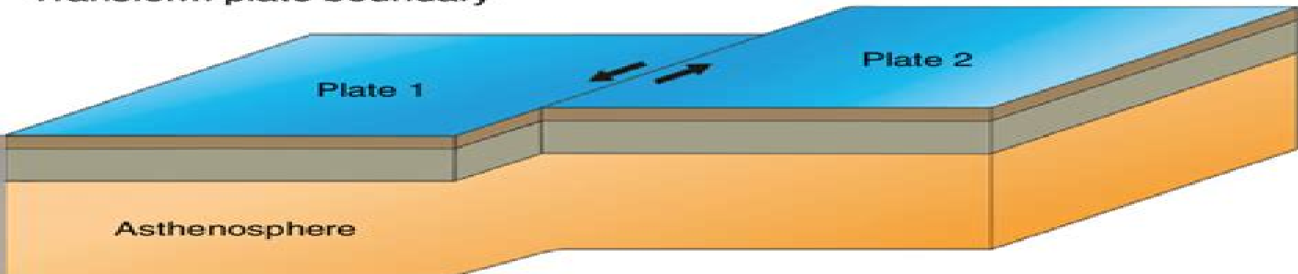
Transform plate boundary
