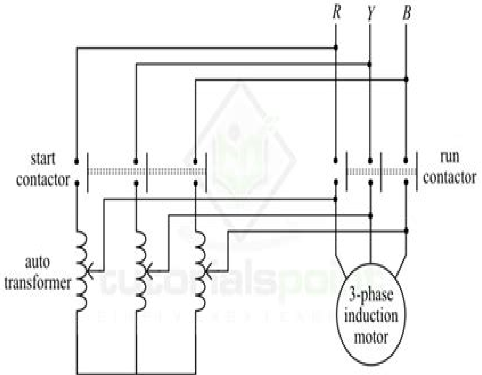
Figure 2 - Autotransformer Starter
