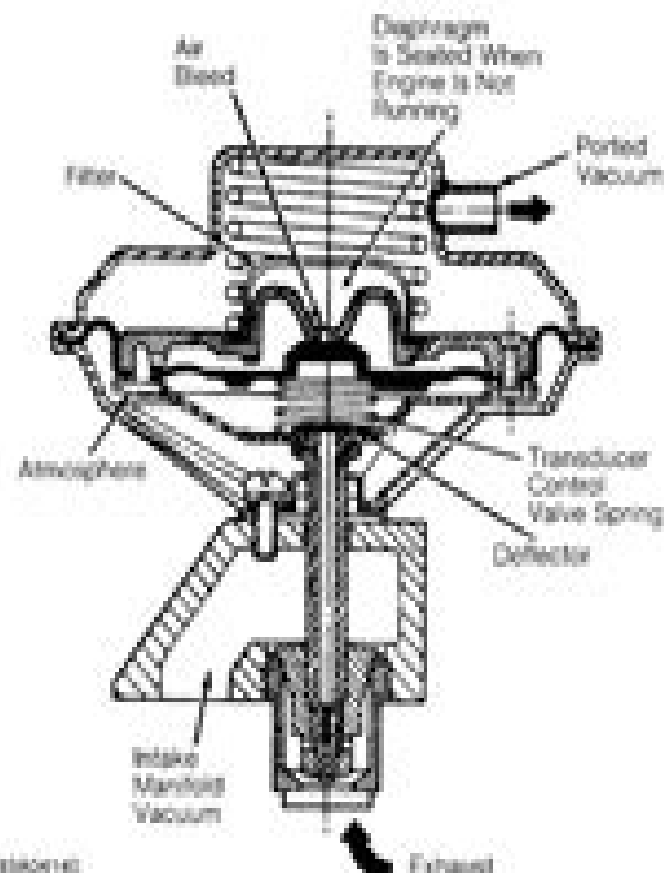
Fig. 9. Typical Negative Backpressure EGR Valve Courtesy of GENERAL MOTORS CORP.
