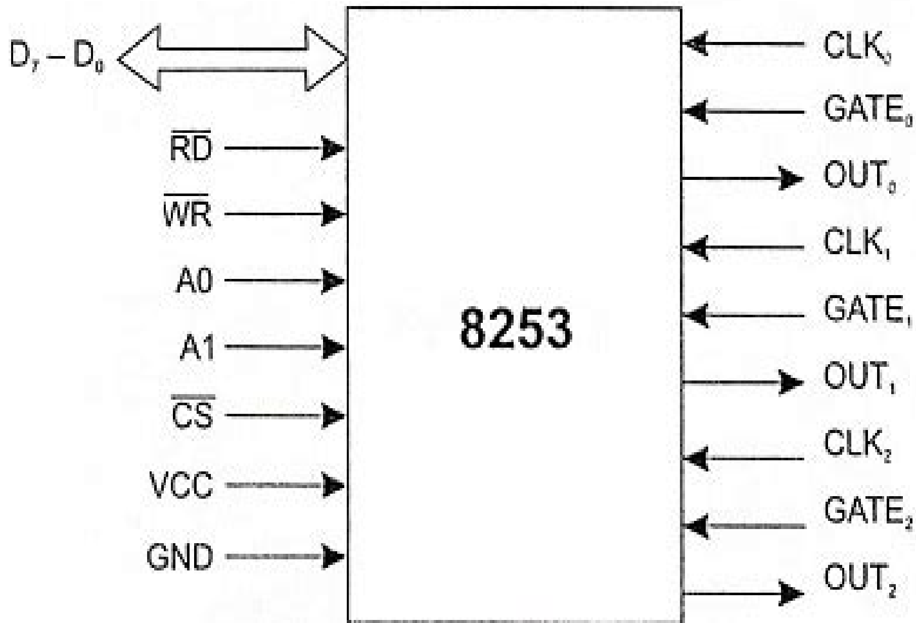
Fig. 8.76 Pin diagram of 8253
