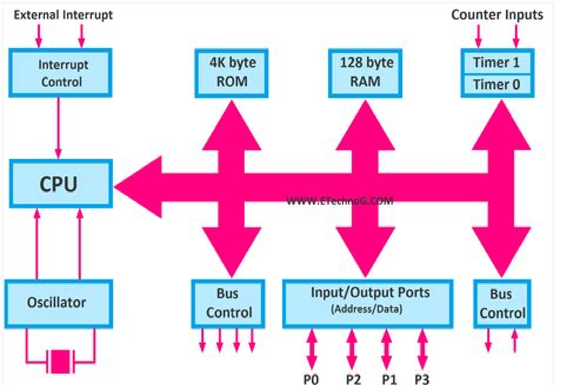
Microcontroller 8051 Architecture and Block Diagram
