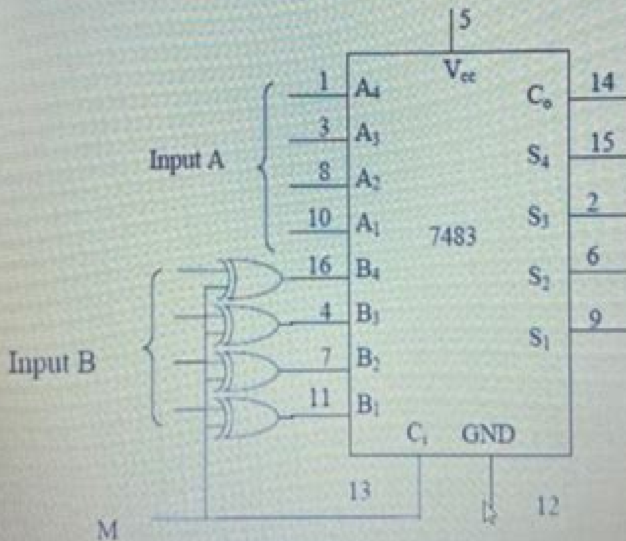
M = 0 for add and M = 1 for subtract Fig.2: 4-bit Binary Adder/Subtractor
