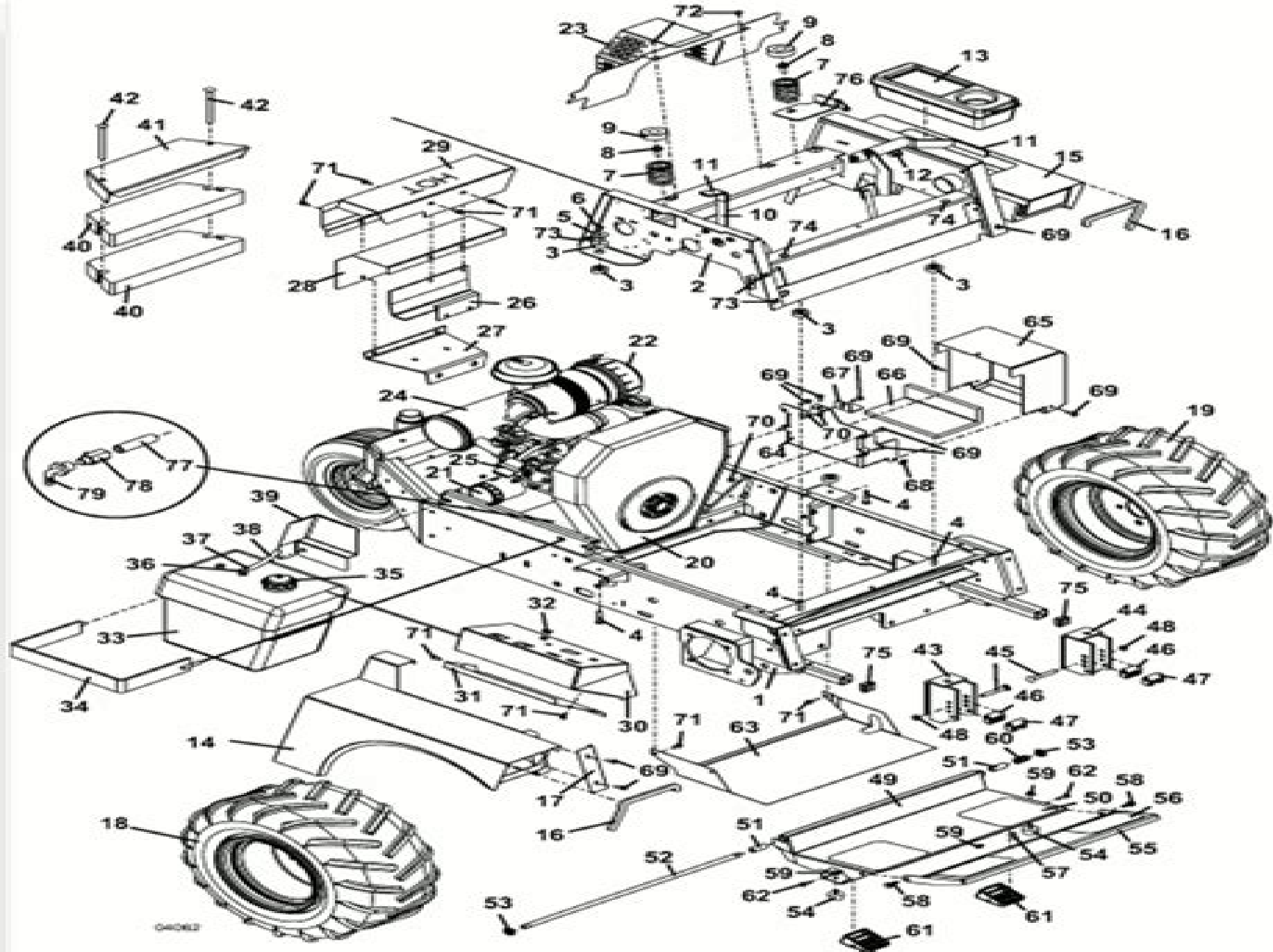
Tractor Assembly
