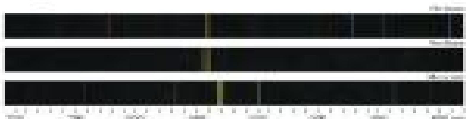
Figure 1. Emission spectrum of the HDL (HDL) under vacuum. The emission lines are shown and the corresponding energy levels (emission spectrum) are shown. The emission lines are shown and the corresponding energy levels (emission spectrum) are shown. The emission lines are shown and the corresponding energy levels (emission spectrum) are shown.
