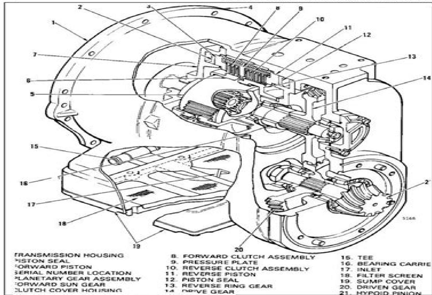
FIGURE 1. POWERSHIFT TRANSMISSION
