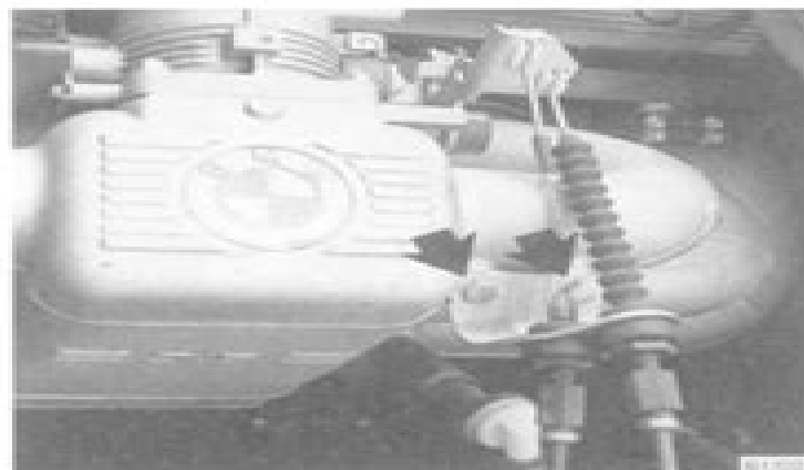
Fig. 25. Throttle, accelerator, and cruise control cable bracket mounting bolts (arrows).
