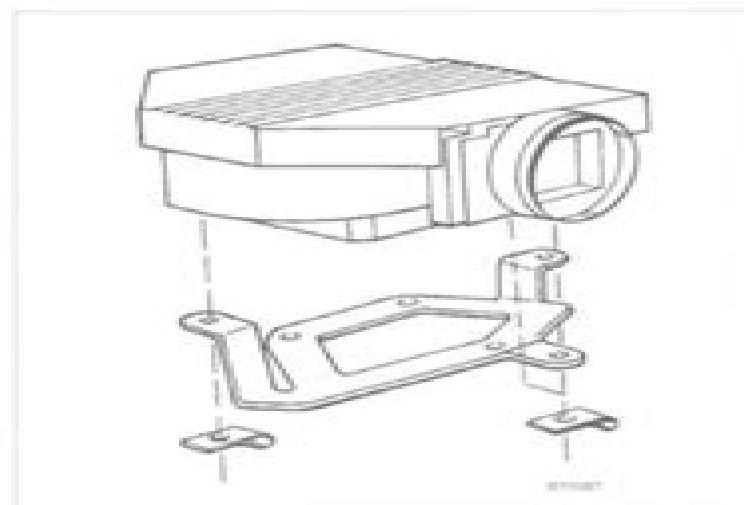
Fig. 26. Air flow sensor retaining clips. Slide clips off pin to remove.
