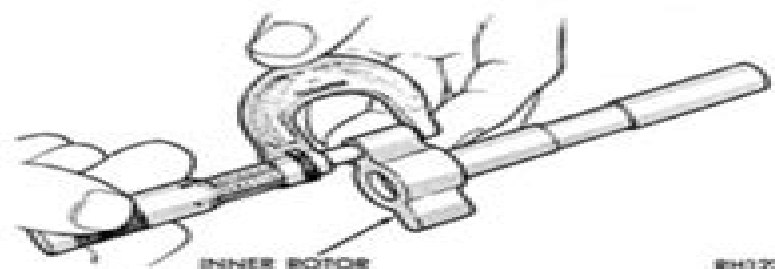
Fig. 43—Measuring Inner Rotor Thickness
