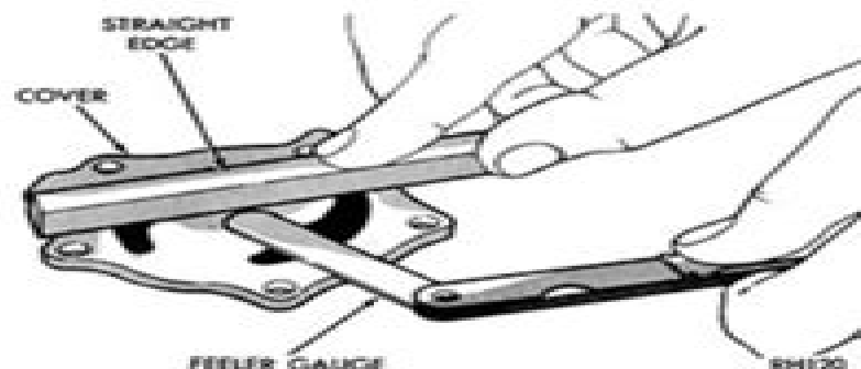
Fig. 41—Checking Oil Pump Cover Flatness
