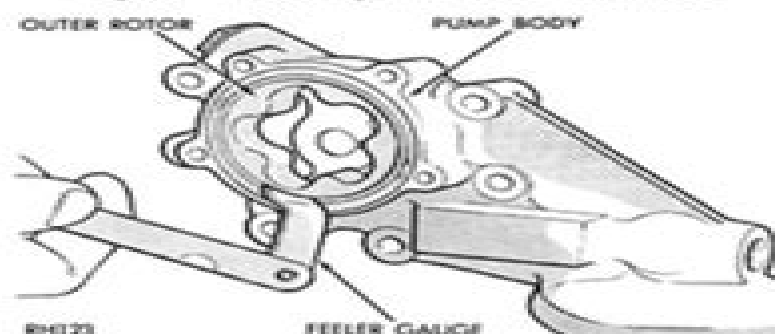
Fig. 44—Measuring Outer Rotor Clearance in Pump Body
