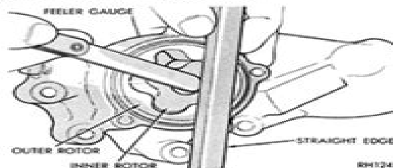
Fig. 45—Measuring Clearance Over Rotors
