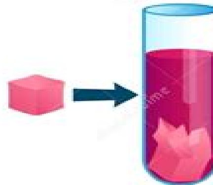
Supersaturated Solution
