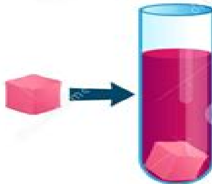
Saturated Solution
