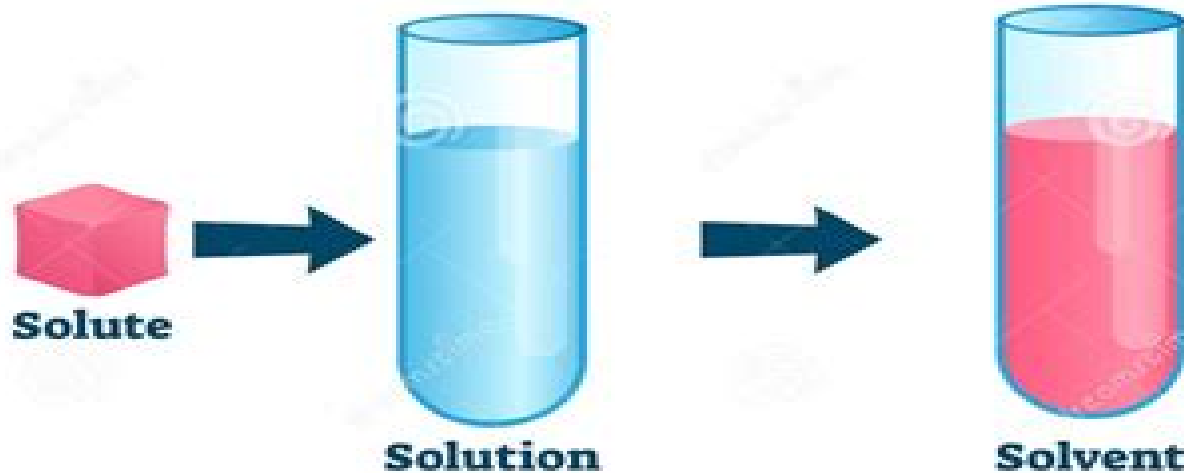
Unsaturated Solution
