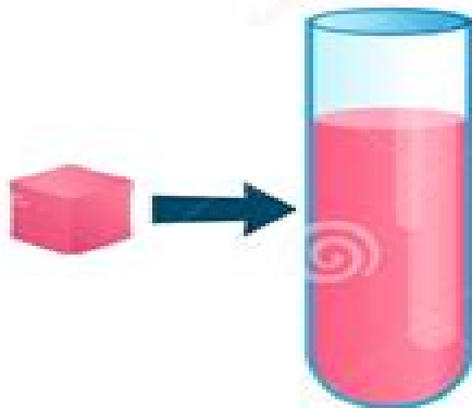
Unsaturated Solution
