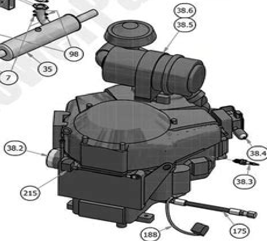
2A - BRIGGS THROTTLE CABLE
