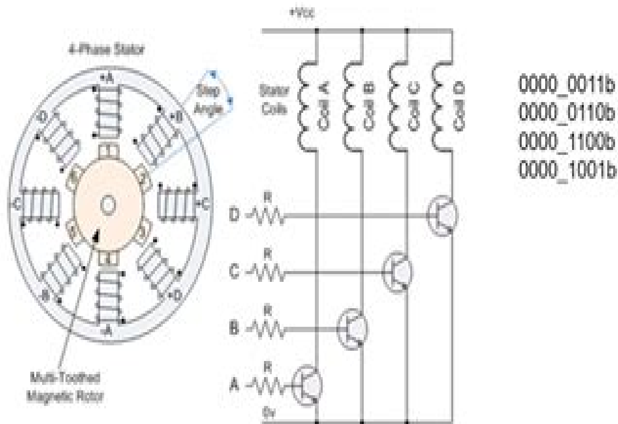
Figure 1: Variable Reluctance
